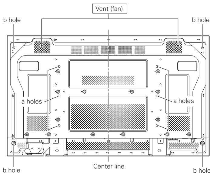
Rear view diagram
